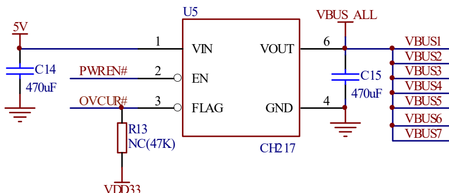
Figure 5-2 overall overcurrent detection and overall power control
